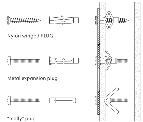
"molly" plug
